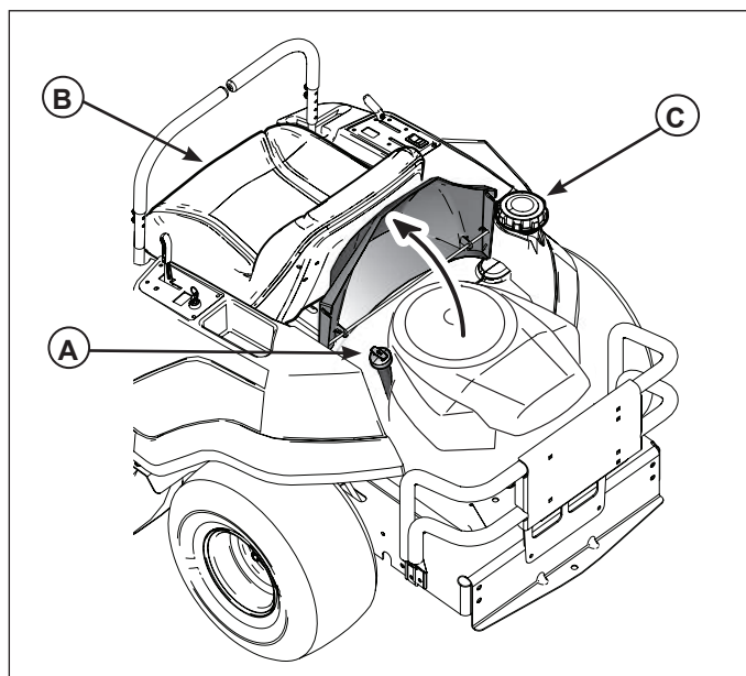
Figure 1. Pre-Start Checks
