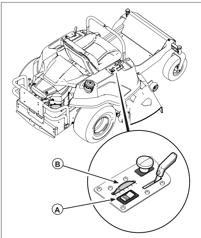
Figure 15. Cutting Height Adjustment
