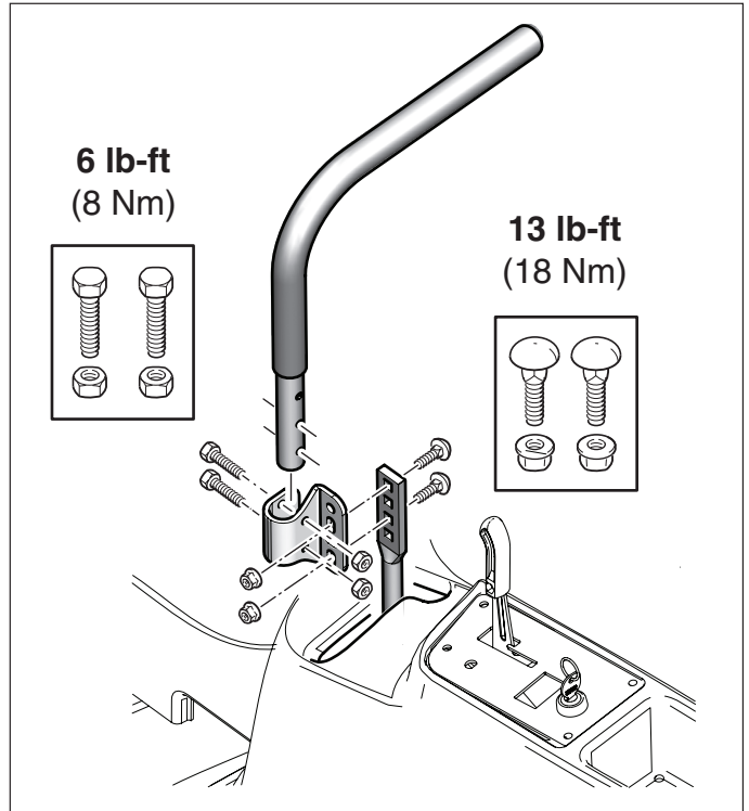
Figure 13. Ground Speed Lever Adjustment
